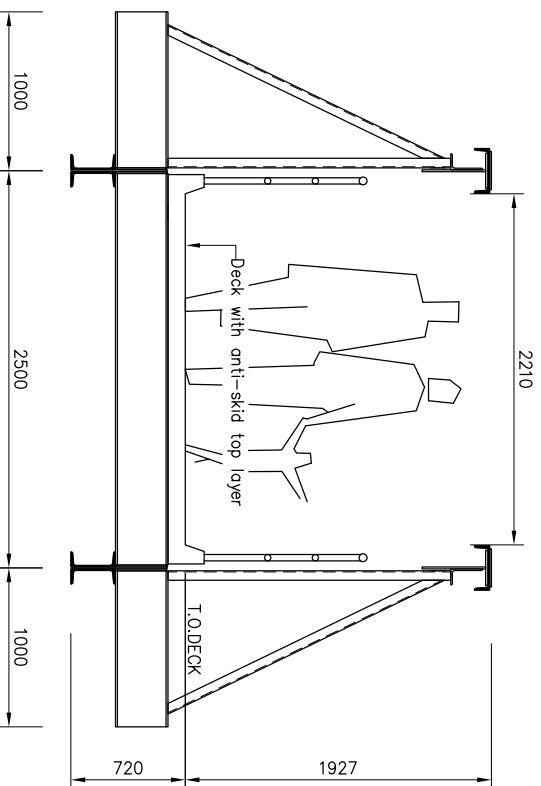
Typ. section of PSB-bridge
