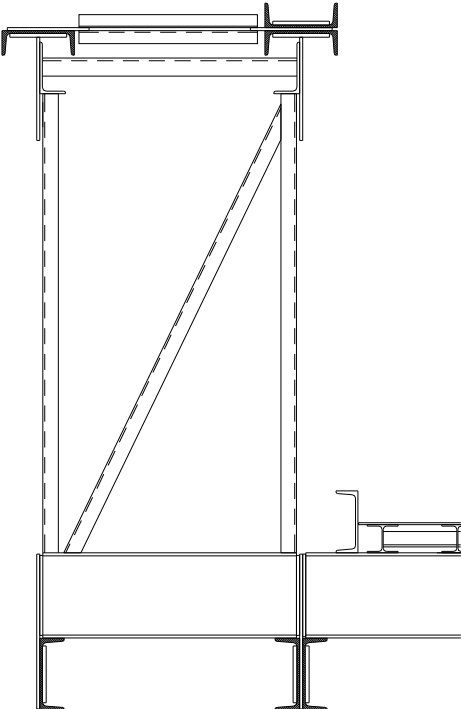
DOUBLE REINFORCED 1
