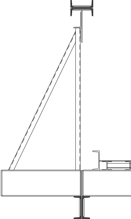
SINGLE REINFORCED
