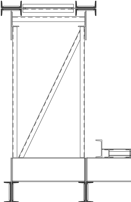
DOUBLE REINFORCED 2
