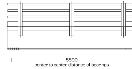
6,00m Free span [1-100]
