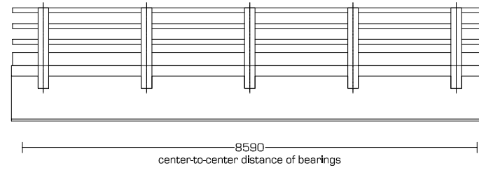
9,00m Free span
