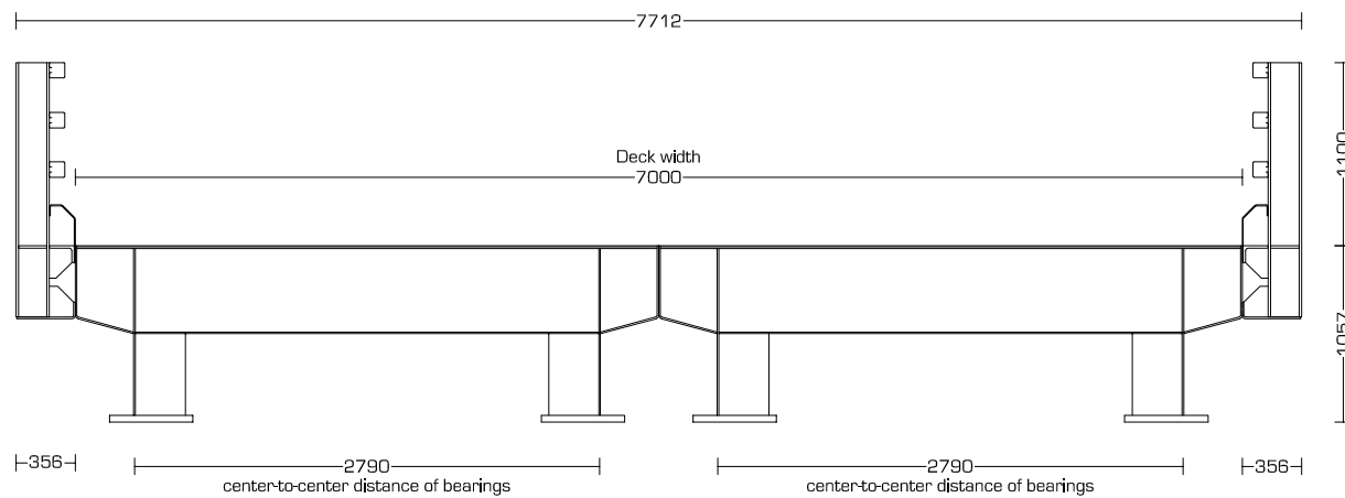
Cross view JSB 100 series - 1,06m Construction height
