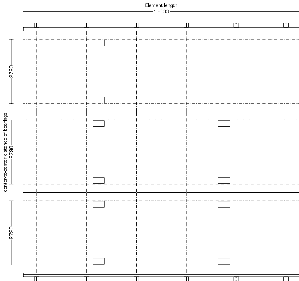
Top view JSB 100 series - 10,50m Deck width [1-100]
