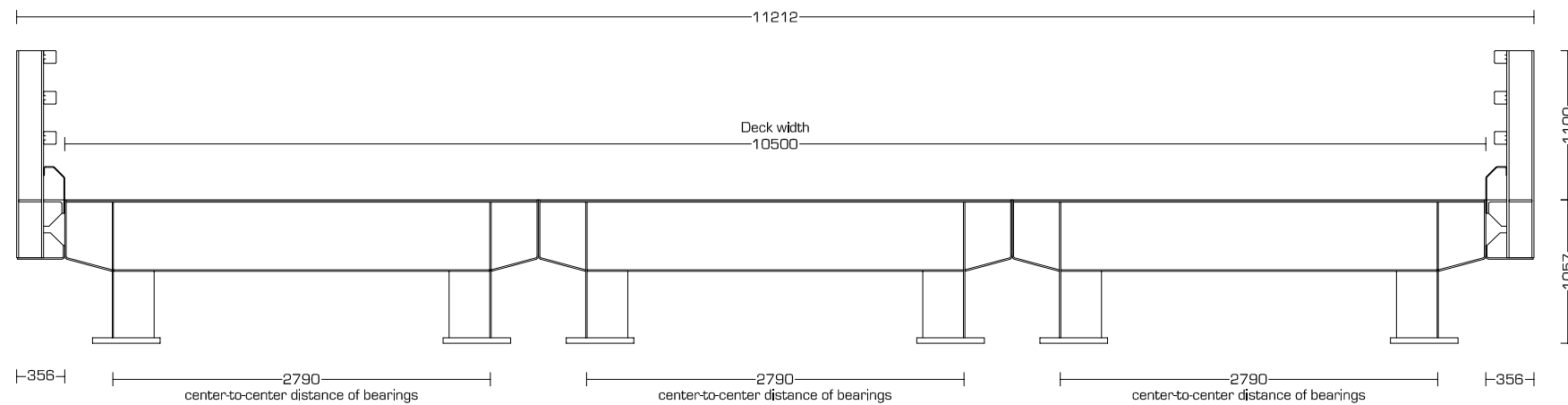
Cross view JSB 100 series - 1,06m Construction height
