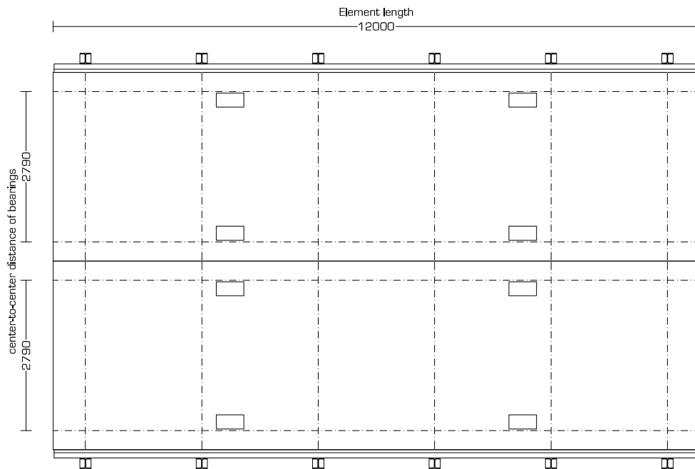
Top view JSB 100 series - 7,00m Deck width [1-100]
