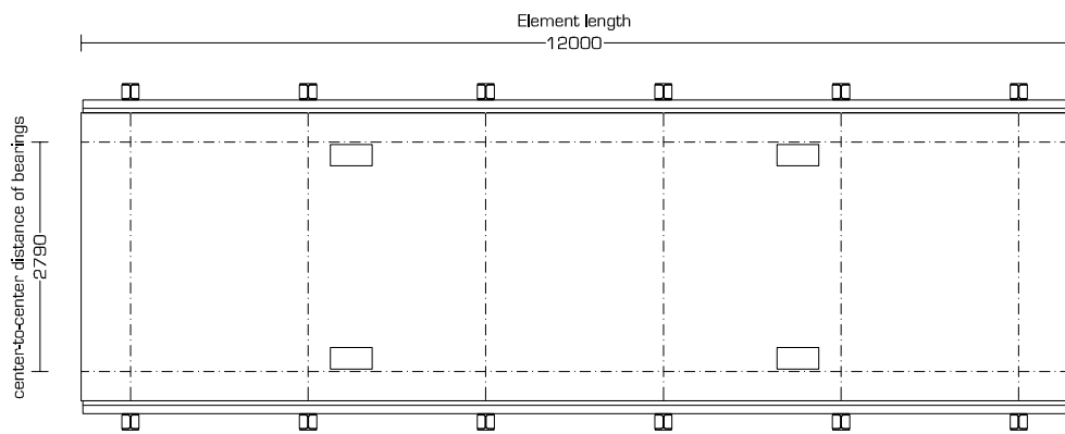
Top view JSB 100 series - 3,50m Deck width [1-100]
